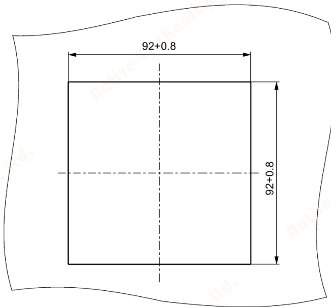
Figure 10-1 Panel cutout
