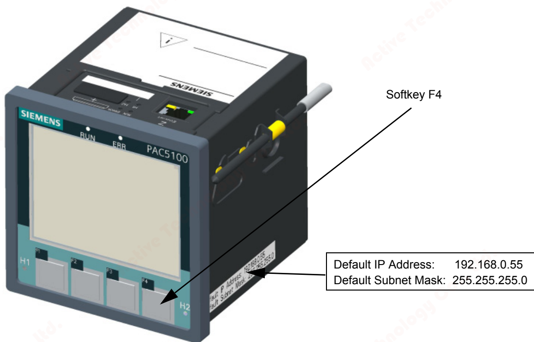
Figure 1-1 Display Side with Softkey F4
