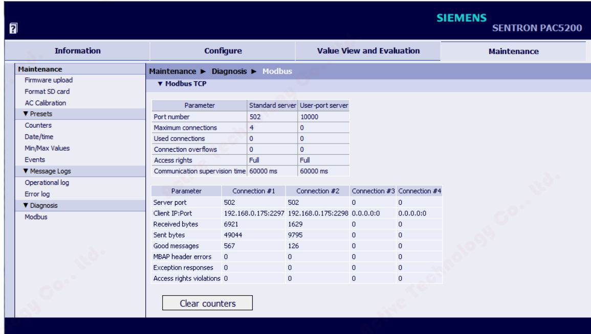
Figure 1-3 Modbus TCP Diagnosis
